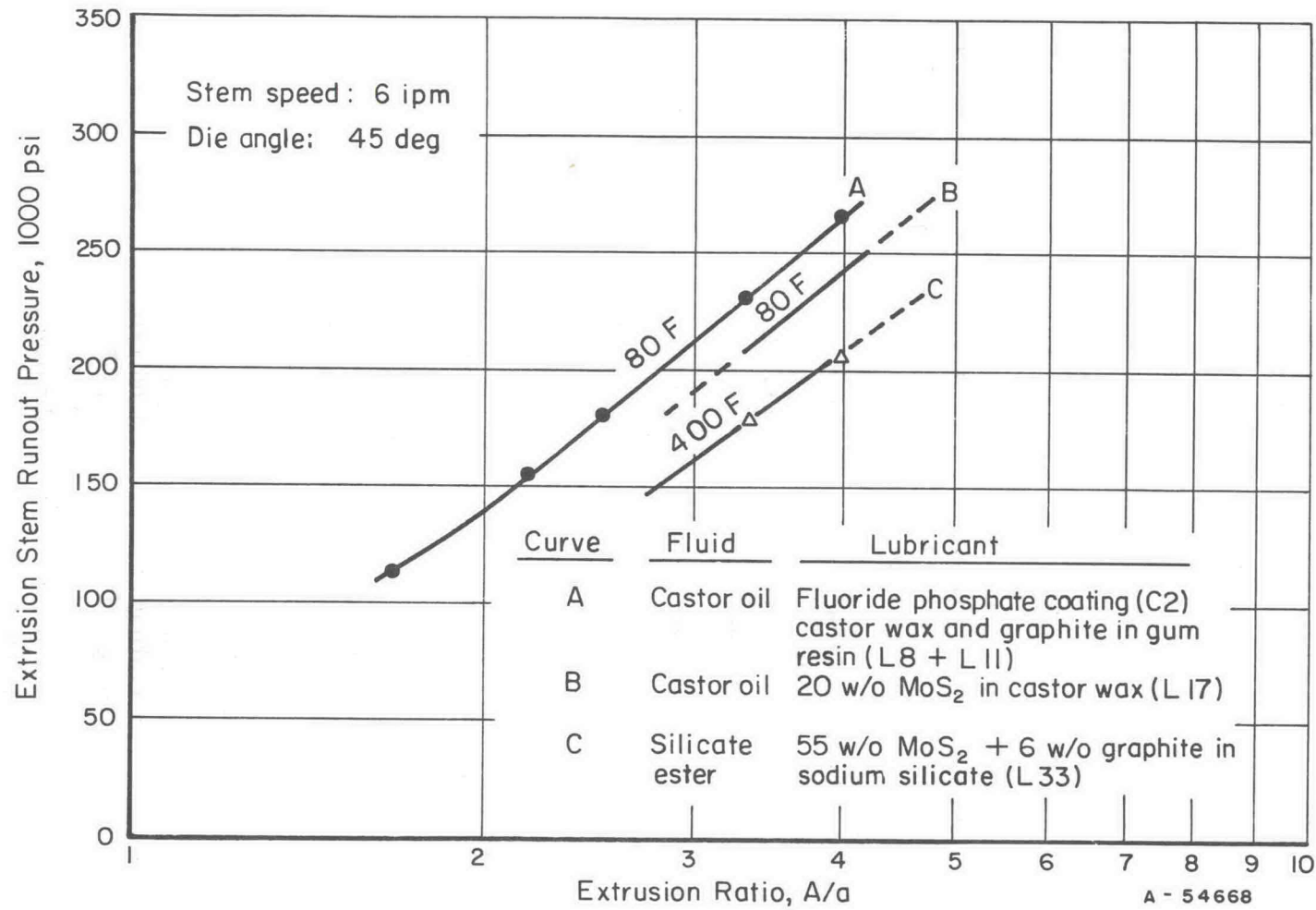
FIGURE 6. COMPARISON OF PRESSURES FOR THE HYDROSTATIC EXTRUSION OF Ti-6Al-4V TITANIUM-ALLOY ROUNDS AT TWO TEMPERATURES
